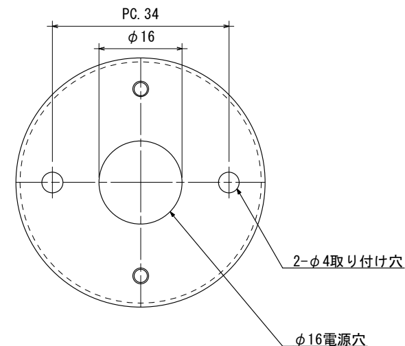
[取付PL-背面図]
