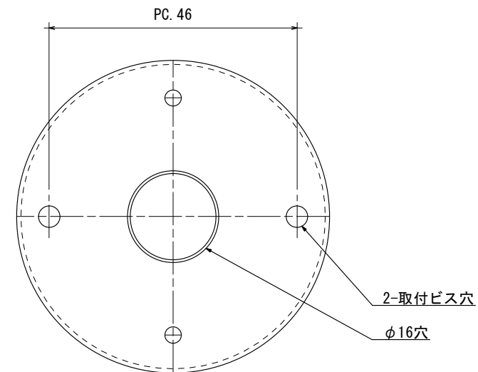
[取付PL-背面図]
